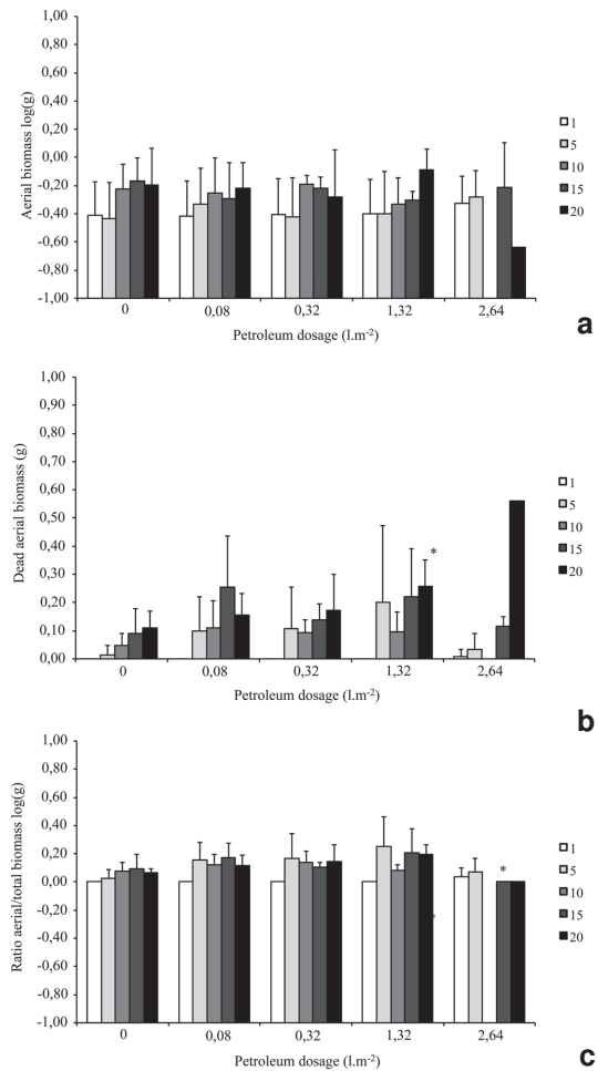
Figure 2 – Effect of Urucu crude oil on Echinochloa polystachya at: a) the aerial biomass (means \pm SD); b) dead aerial biomass (means \pm SD); c) the ratio of aerial live/total biomass (means \pm SD). * significant difference ( \alpha = 0.05 ) compared to the control.
