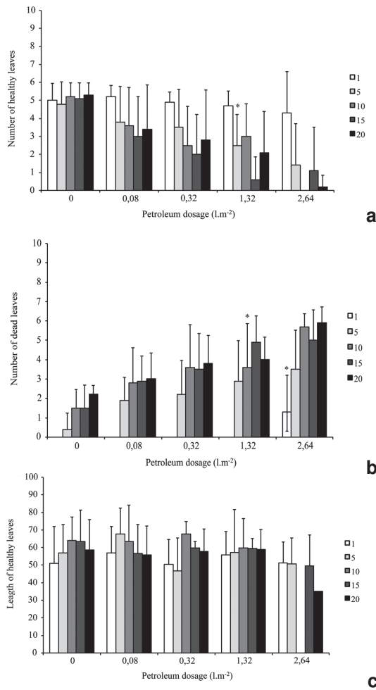
Figure 1 – Effect of Urucu’s oil over Echinochloa polystachya at: a) the number of healthy leaves (means \pm SD); b) the number of dead leaves (means \pm SD); c) the length of healthy leaves (means \pm SD). * significant difference ( \pm = 0.05 ) compared to the control.
